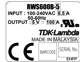
SCALE FOR NAME PLATE : 2/1
