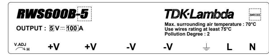
SCALE FOR NAME PLATE : 1/1
