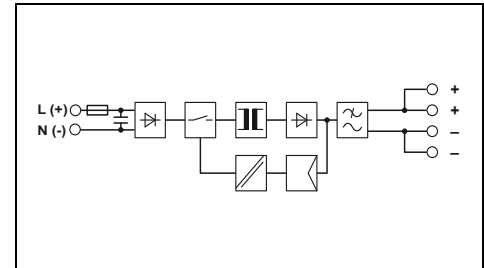
Power supply, 1 AC, 24 V DC, 3.5 A Input up to 277 V AC, NEC Class 2
