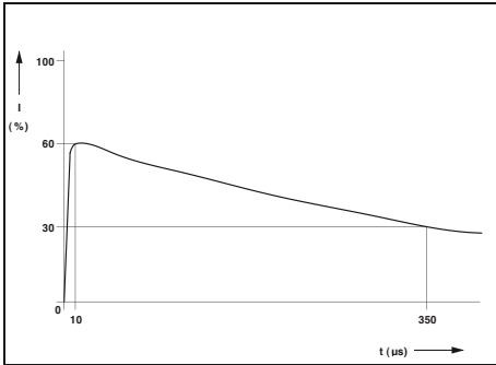
10/350 lightning current pulse according to IEC 62305-1
