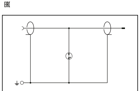
For GSM systems (0 - 6 GHz), grounded shield, connection: type N
