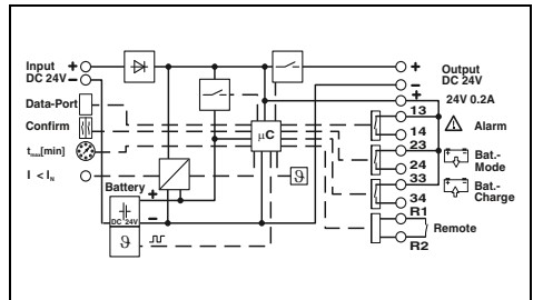
Uninterruptible power supply with integrated power storage, 24 V DC / 24 V DC, 10 A, 3.4 Ah
