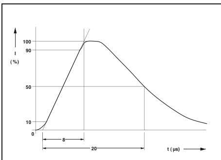
8/20 surge current pulse according to IEC 60060-1
