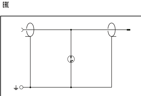
For GSM systems (0 - 3 GHz), grounded shield, connection: N type
