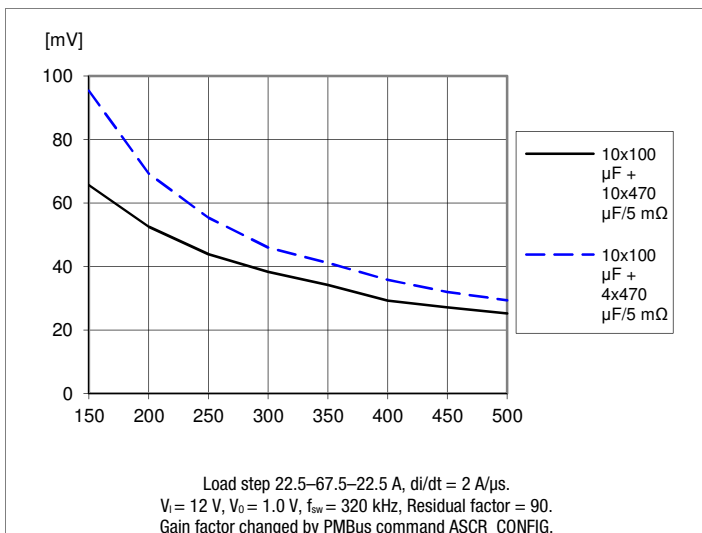
Voltage deviation vs. control loop gain setting and output capacitance.
