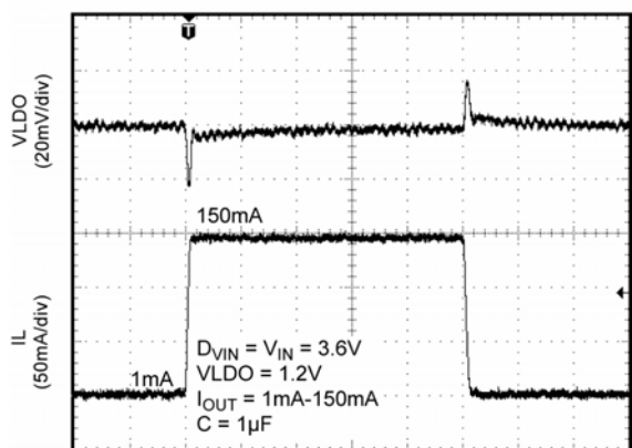
LDO Load Transient
