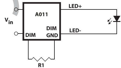
Figure 19. Using resistor for fixed current reduction Output is approximately: \%I_{OUT} = R1/200 EG: 10K \approx 50%
